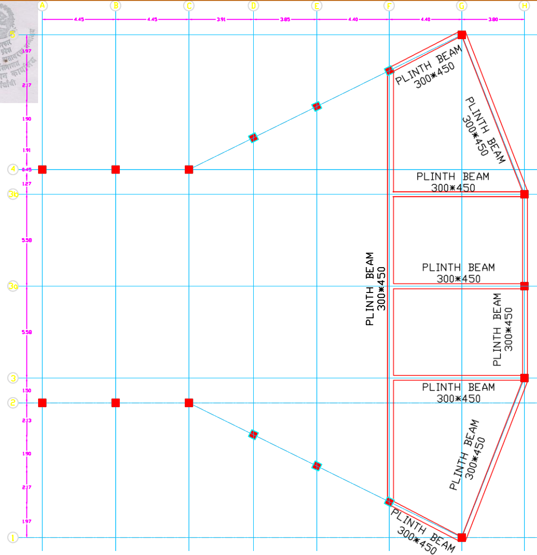
PLINTH BEAM LAYOUT PLAN AT+3.1 LEVEL
