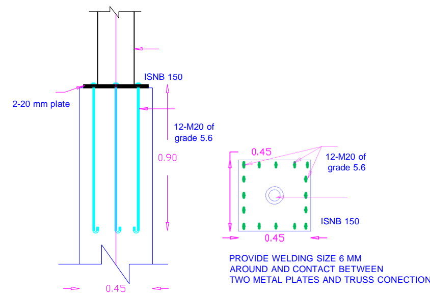
BASE AND BOLTS SECTION
