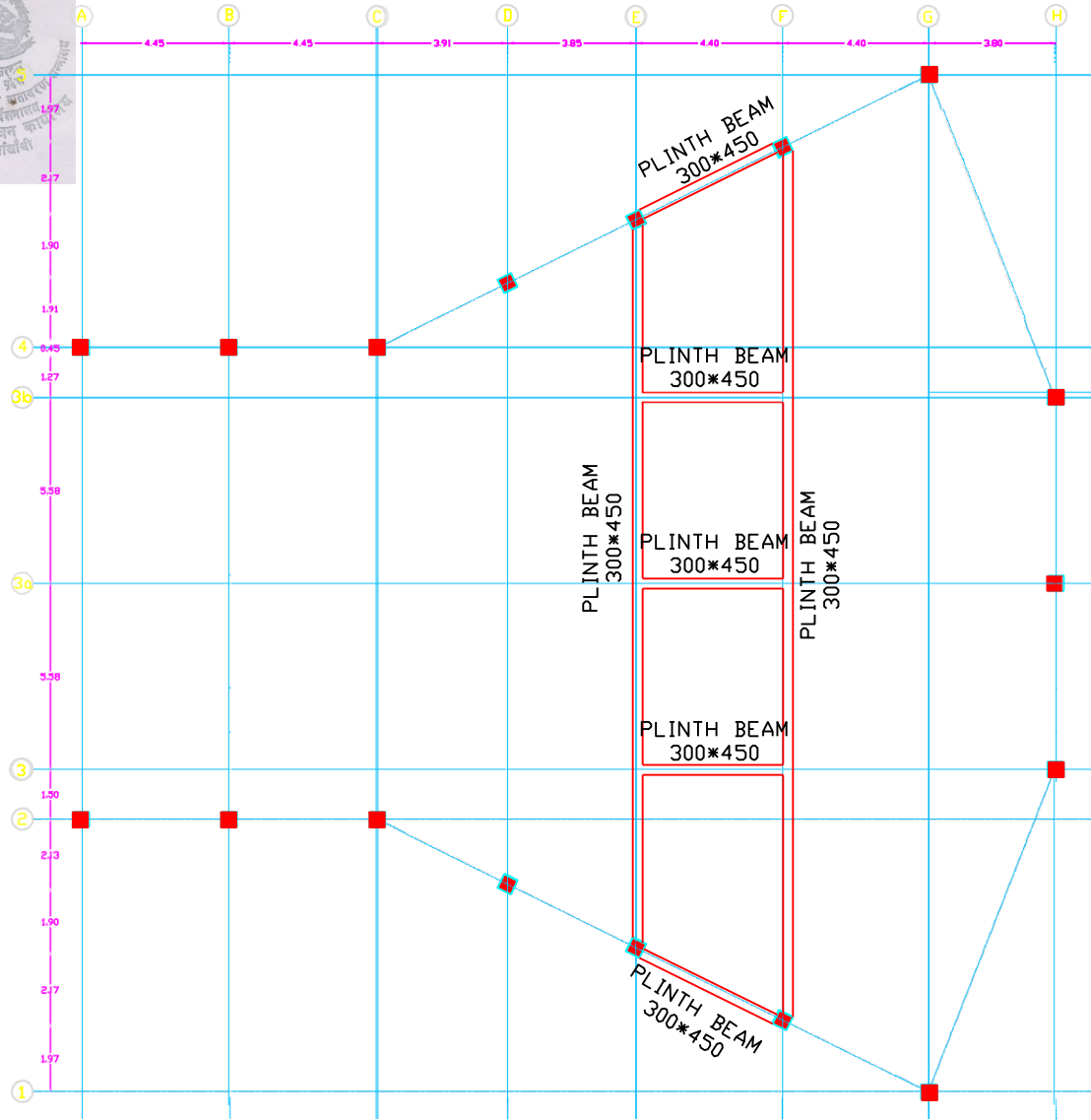
PLINTH BEAM LAYOUT PLAN AT+2.4 LEVEL
