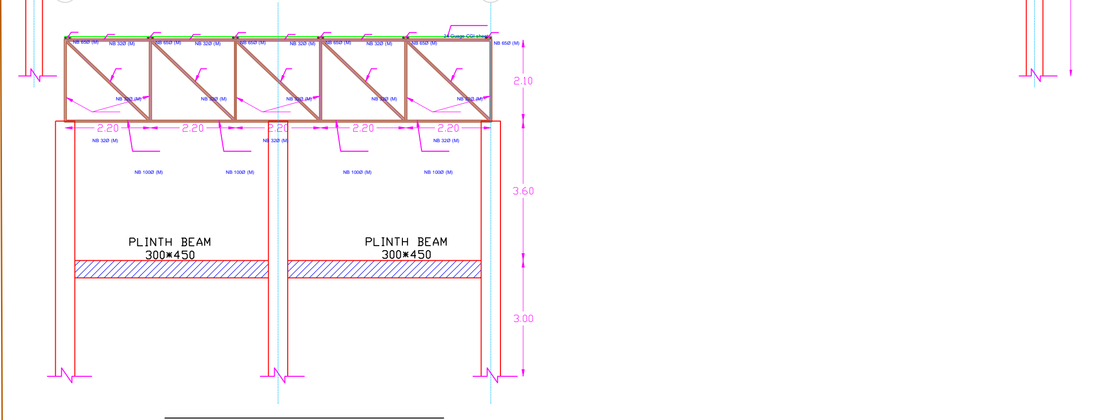
TRUSS T6 SECTION ALONG GRID H
