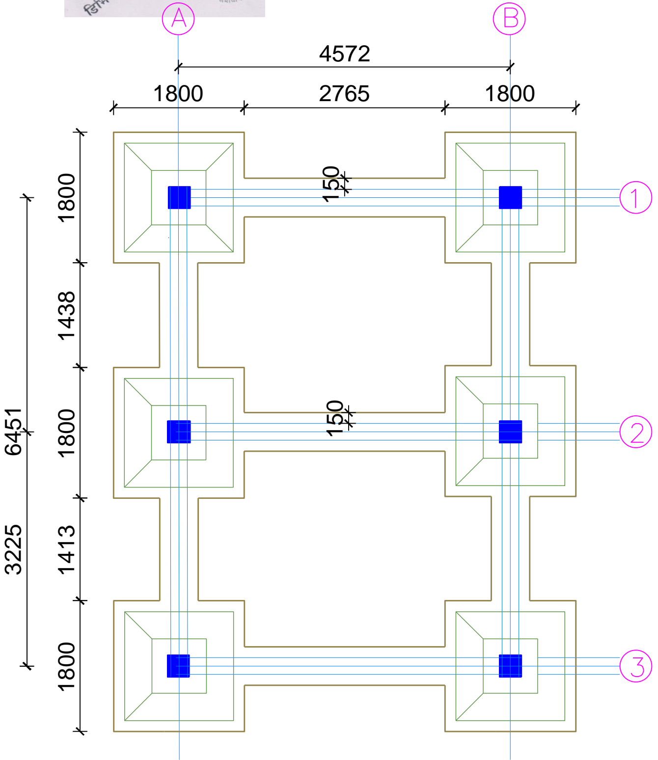
Foundation Layout Plan
