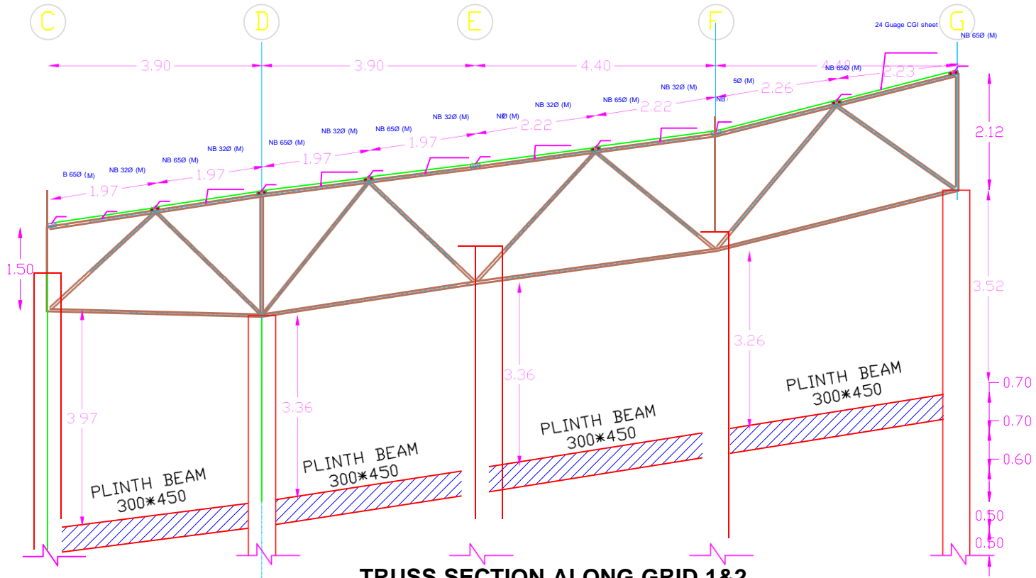
TRUSS SECTION ALONG GRID 1&2 Scale:-1:40
