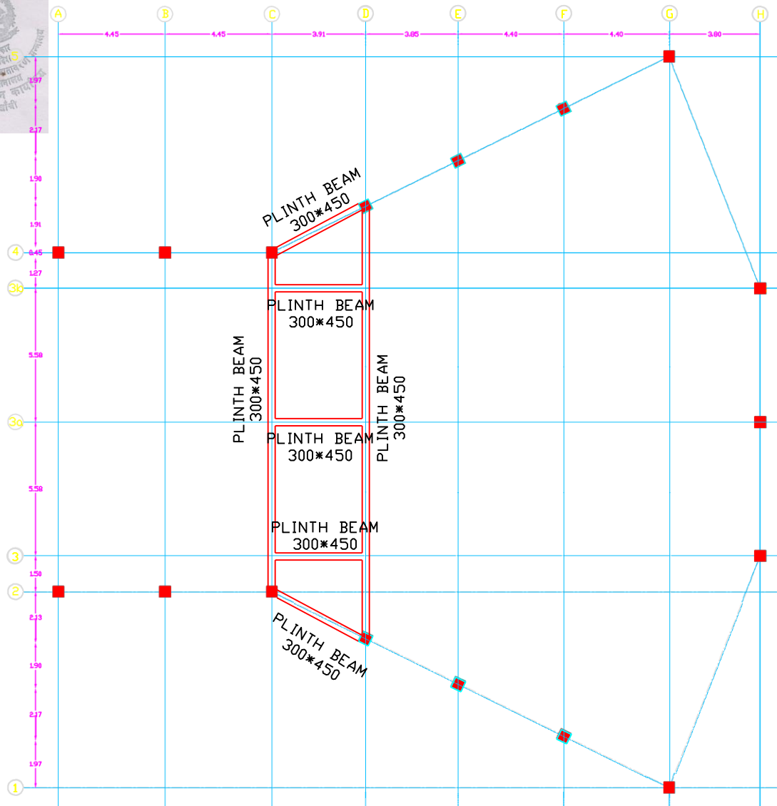
PLINTH BEAM LAYOUT PLAN AT+1.1M LEVEL
