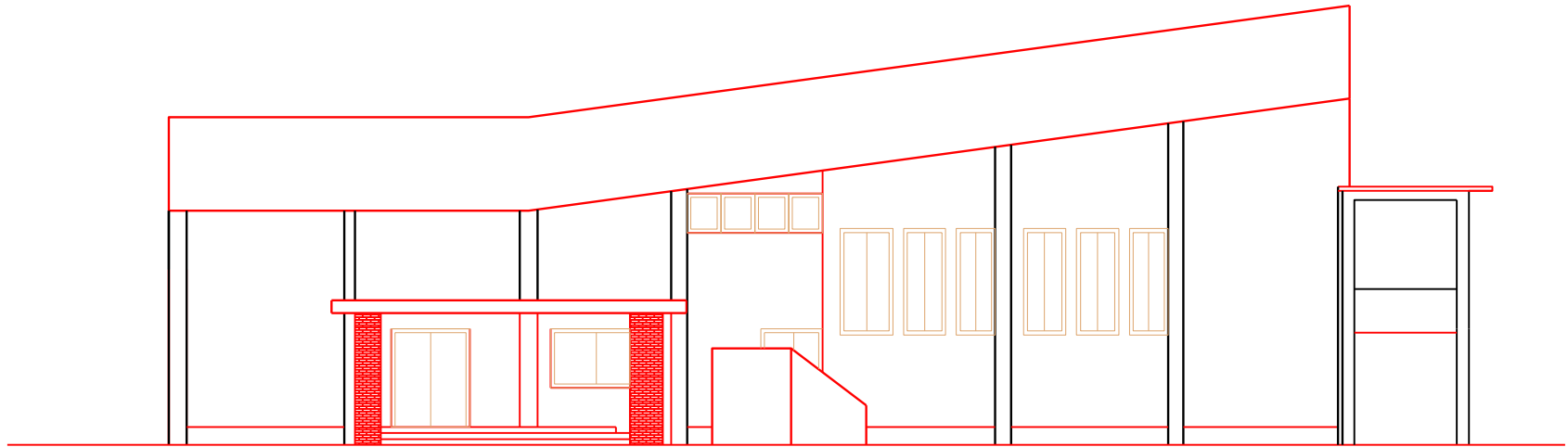
LEFT ELEVATION
