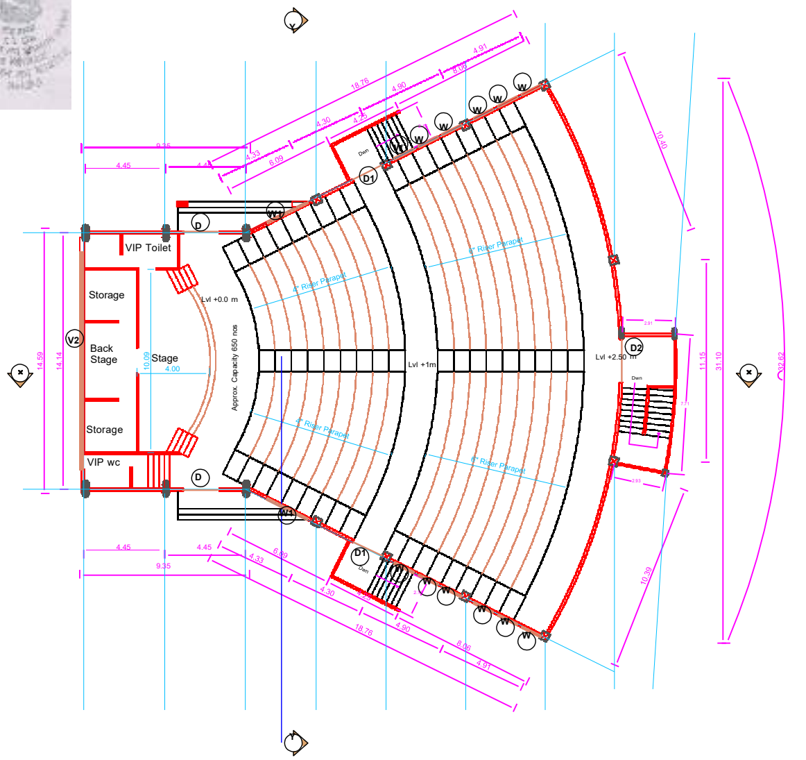
FLOOR PLAN AREA: 600.19 SQM
