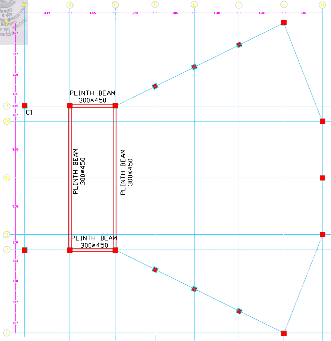
PLINTH BEAM LAYOUT PLAN AT+0.5M LEVEL
