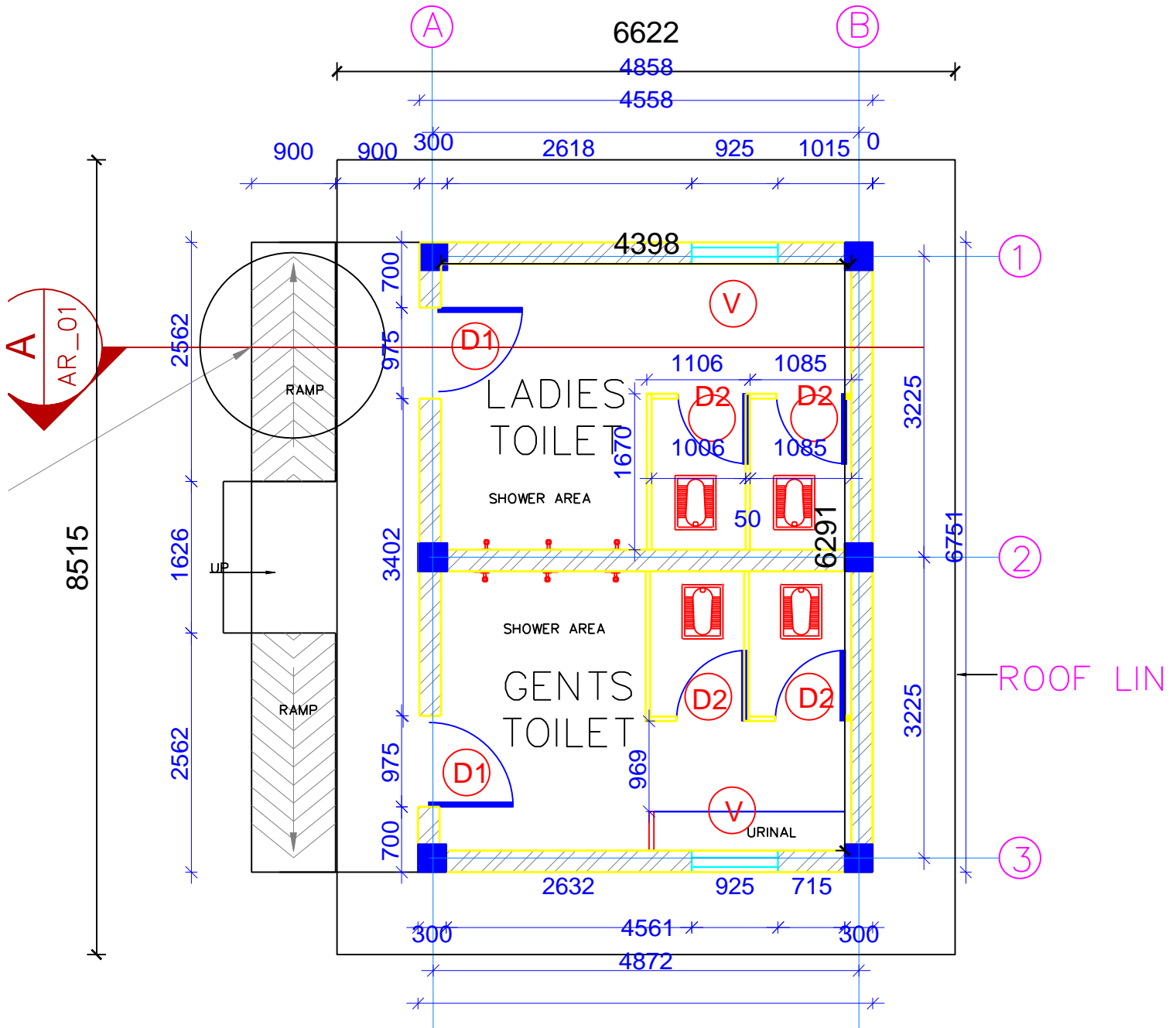
GROUND FLOOR PLAN FLOOR AREA: 32.88 SQ. M.
