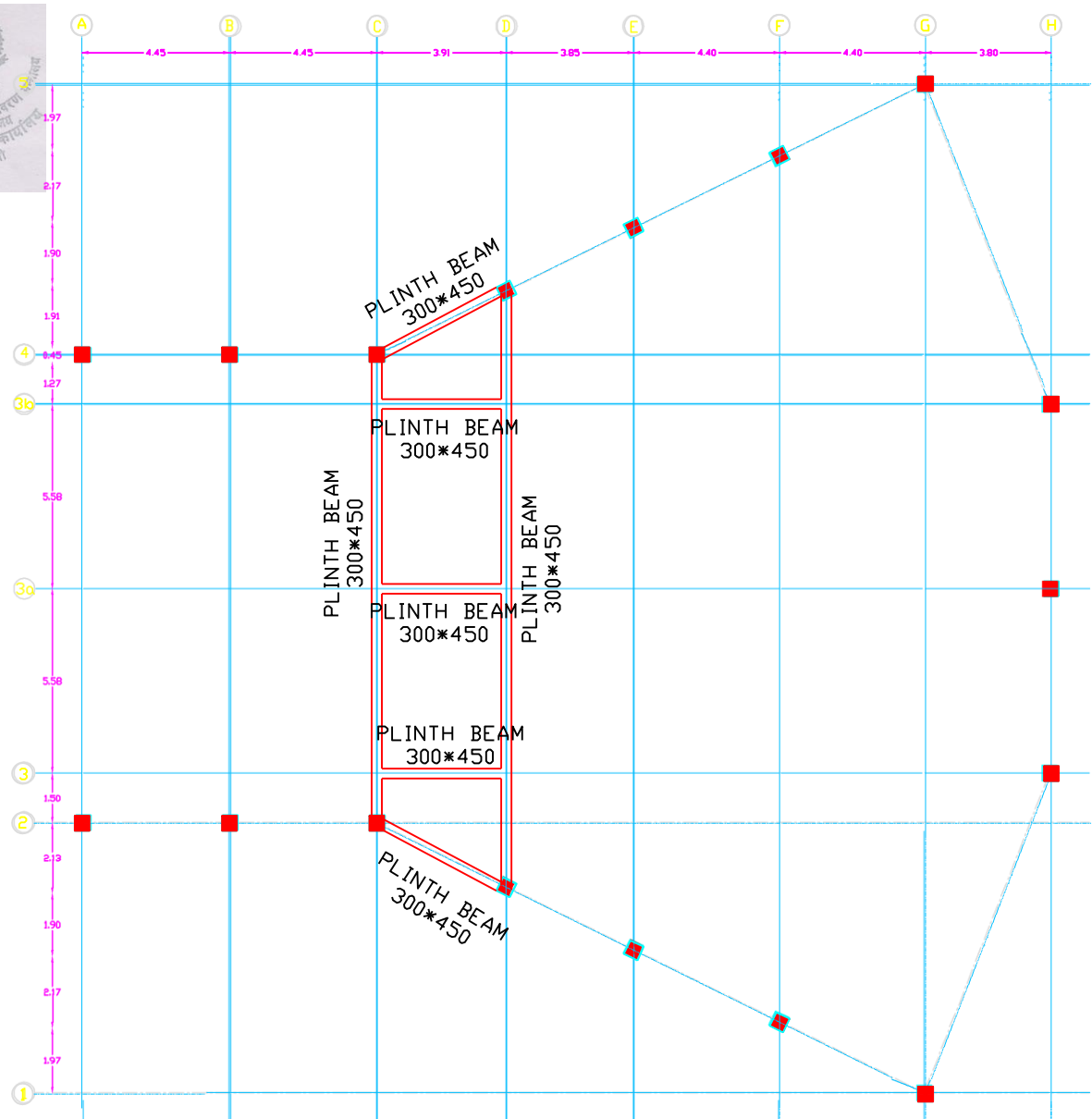
PLINTH BEAM LAYOUT PLAN AT+1.1M LEVEL
